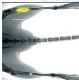
Spectral unmixing
