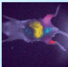
Multiwavelength fluorescence
